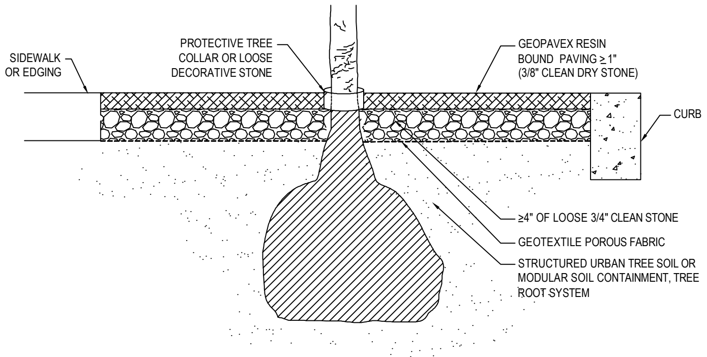
SECTION VIEW
